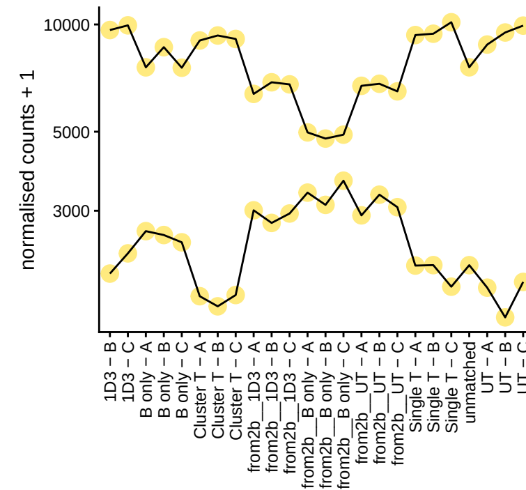
ERV3-1-6 | profile
