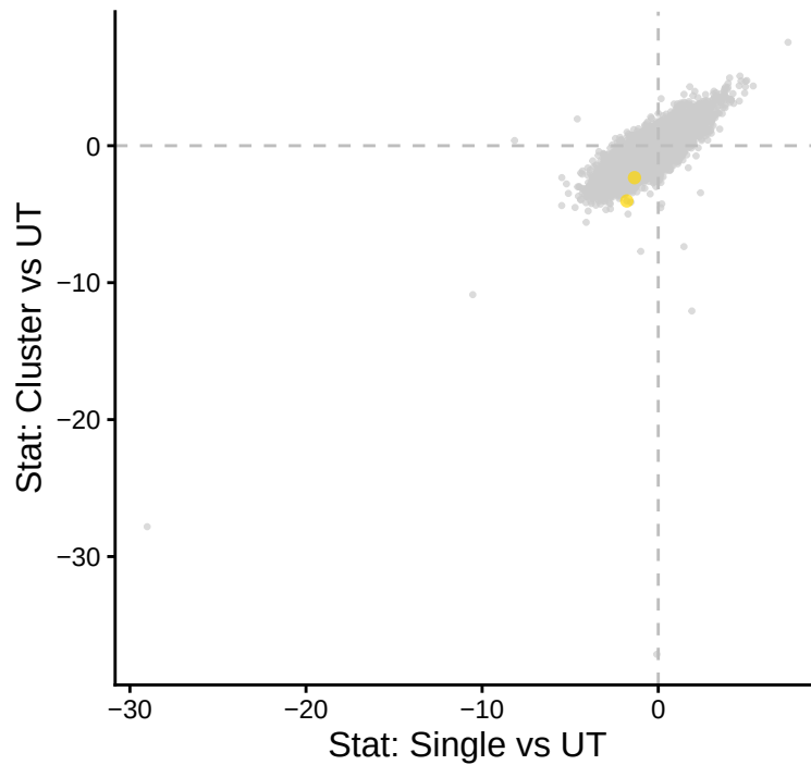
ERV3-1-6 | pools
