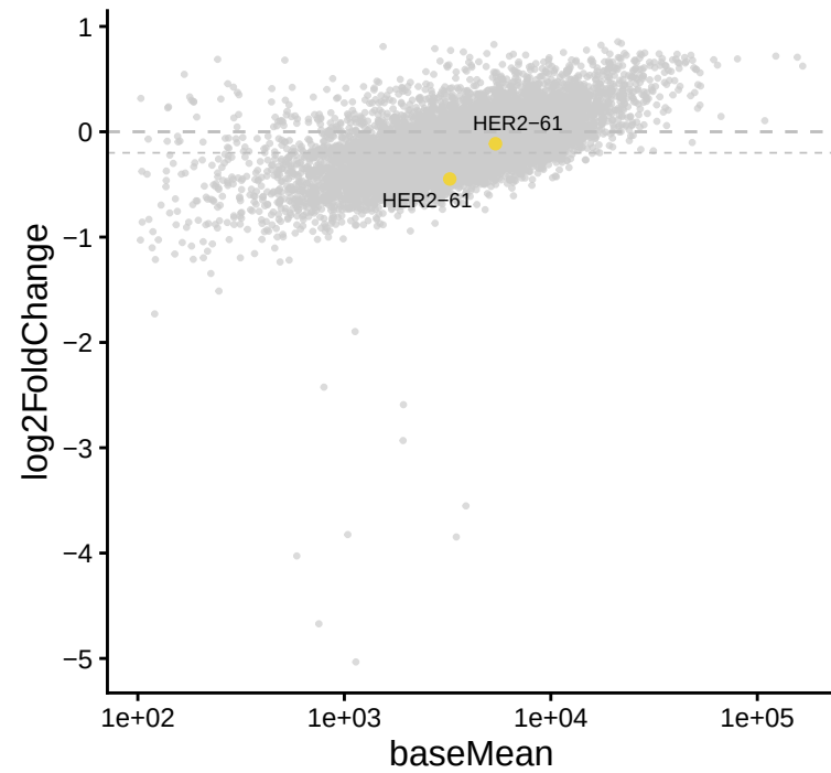
HER2-61 | UT vs B
