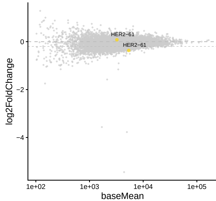
HER2-61 | Cluster vs UT
