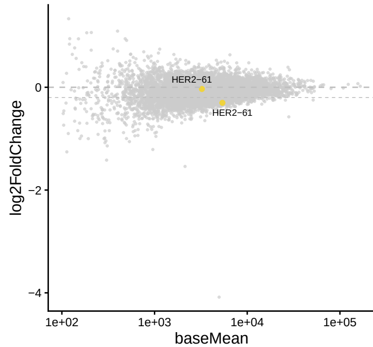
HER2-61 | Single vs UT
