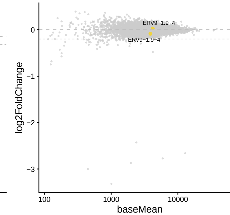
ERV9-1.9-4 | Single vs UT
