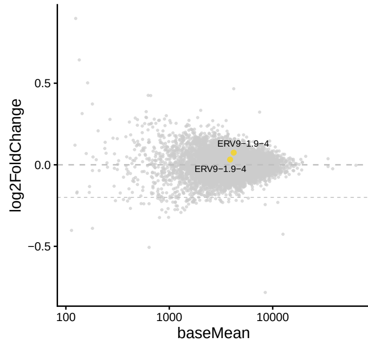
ERV9-1.9-4 | UT vs B
