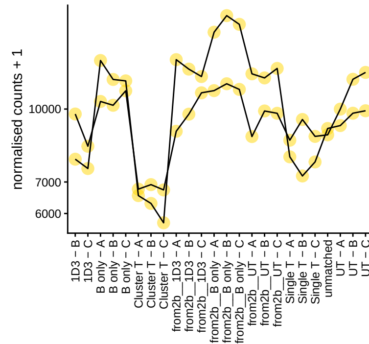
FLU_NP-17 | profile
