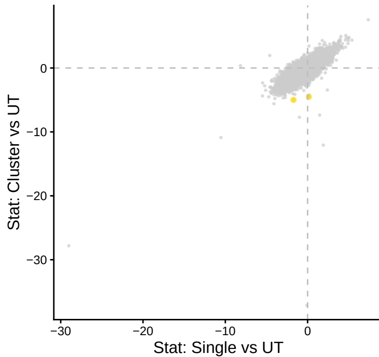
FLU_NP-17 | pools
