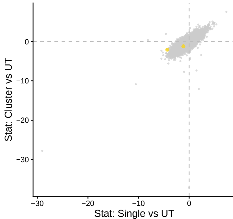
ERVK-9.4-6 | pools
