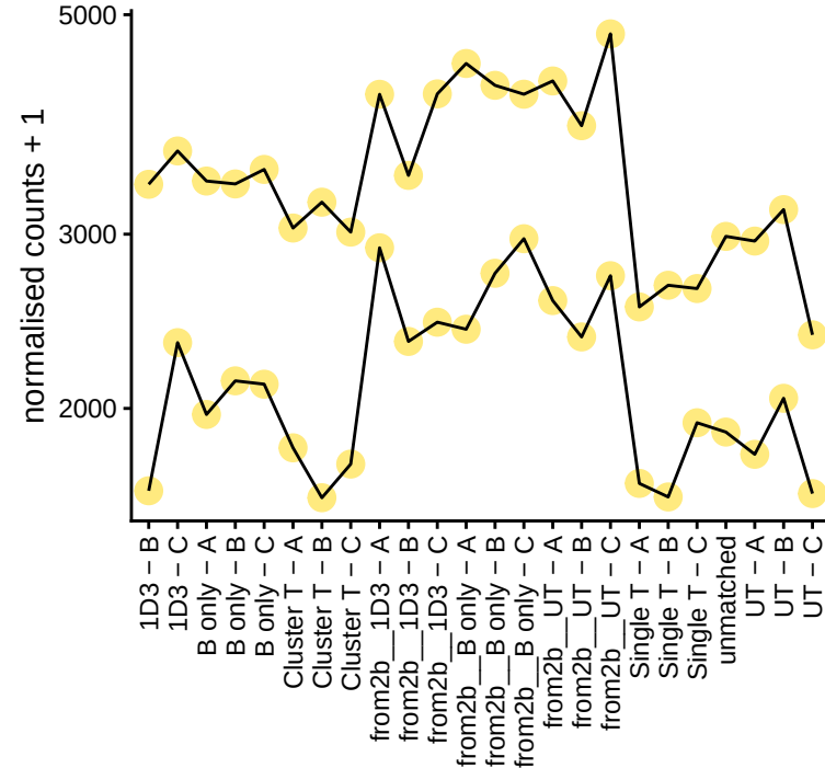
ERVK-9.4-6 | profile
