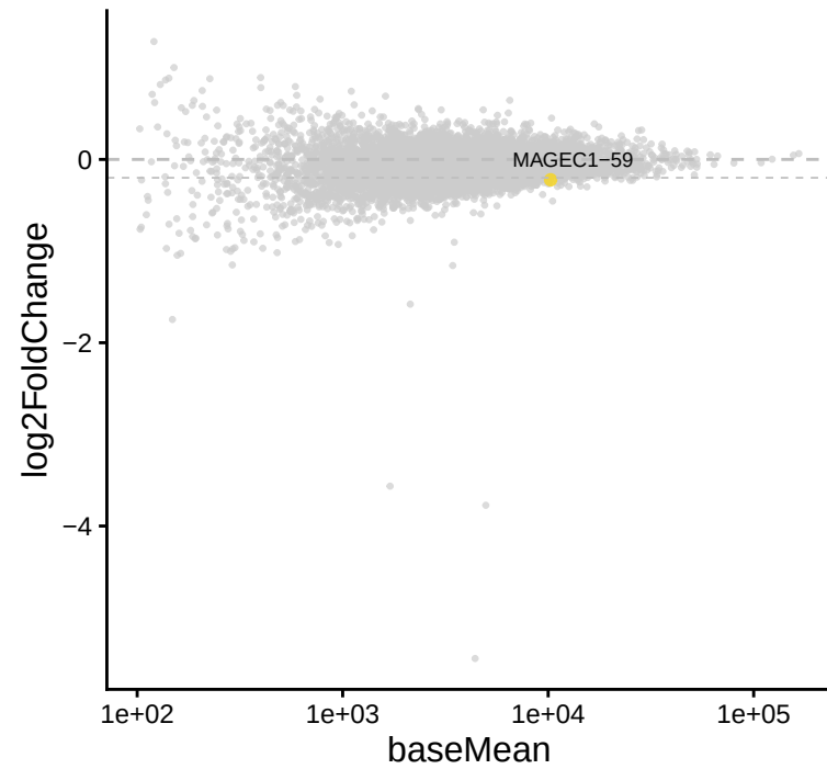
MAGEC1-59 | Cluster vs UT
