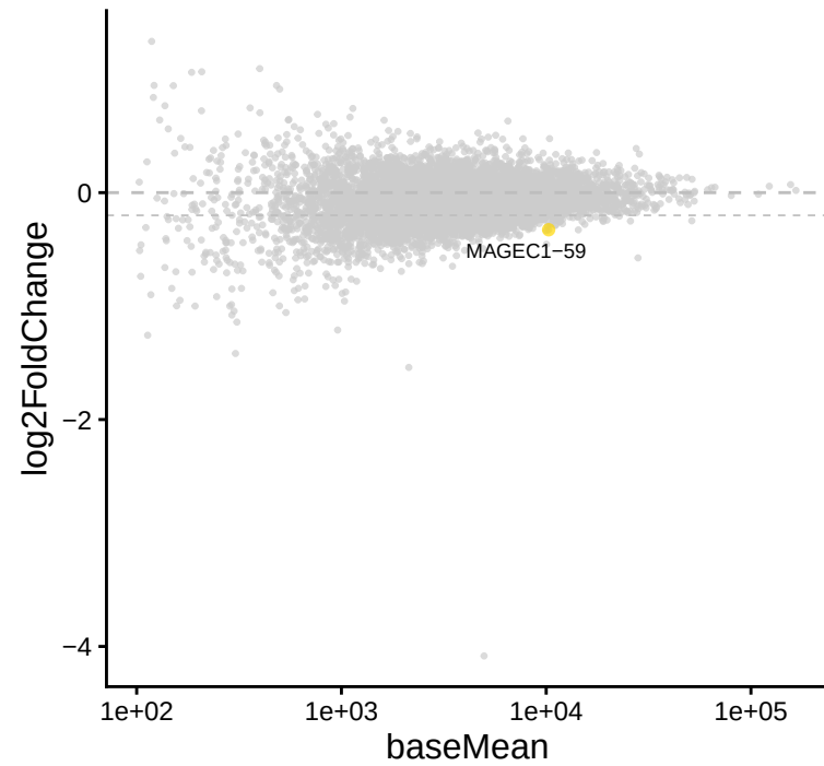
MAGEC1-59 | Single vs UT
