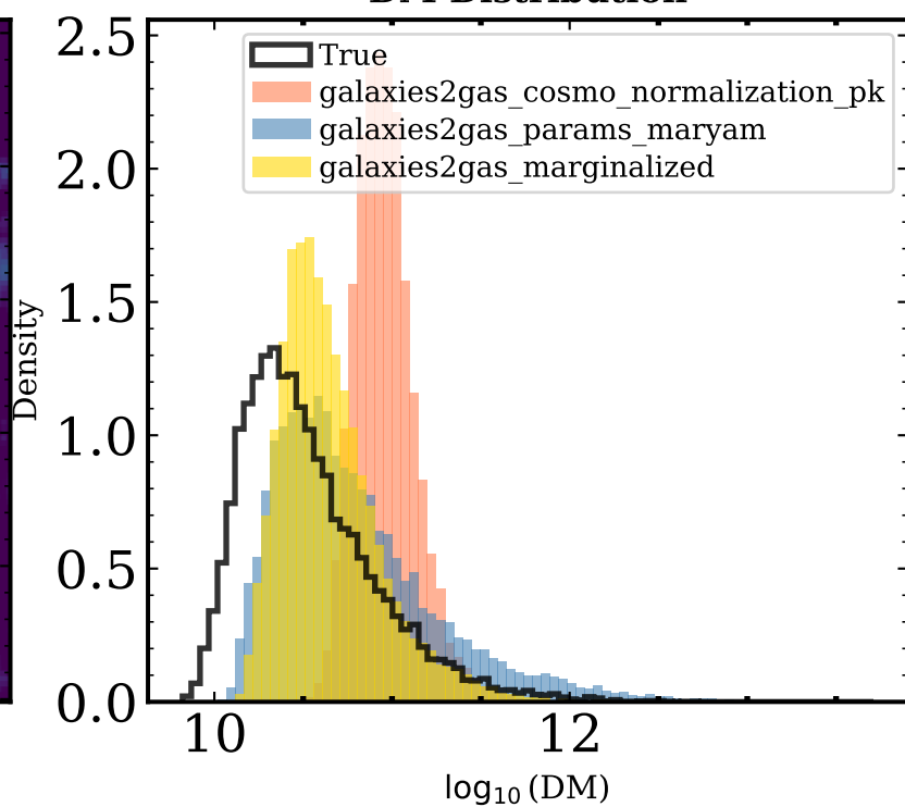
DM Distribution
