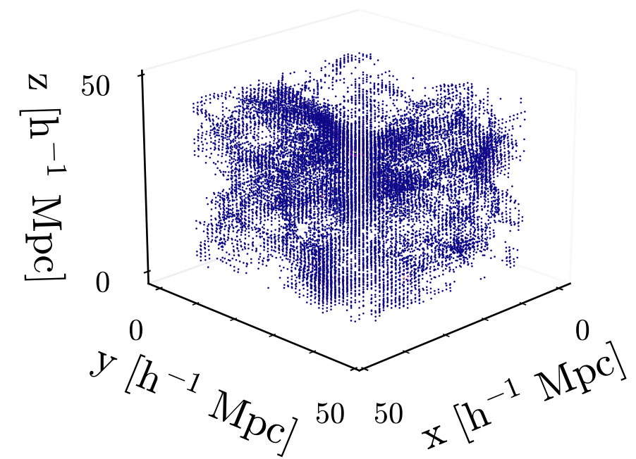
Reconstructed Gas
