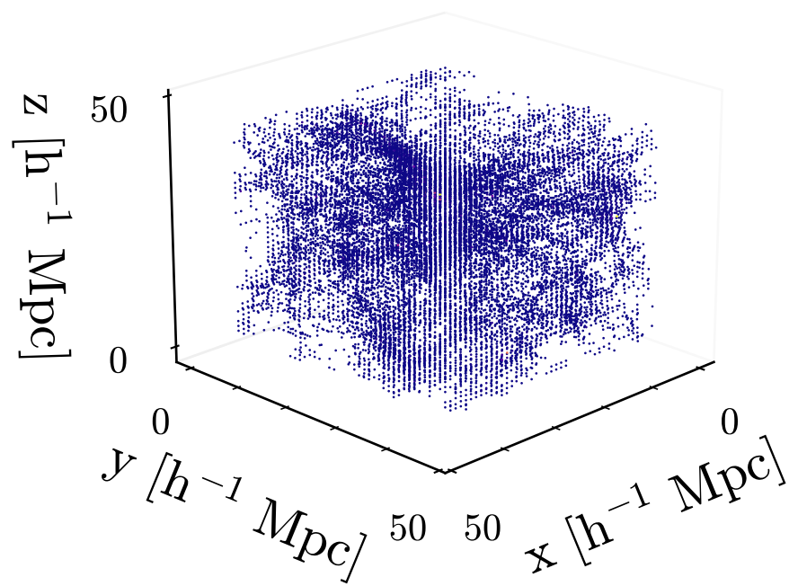
True Gas
