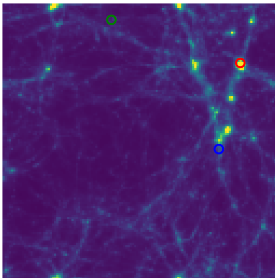
Truth DM map
