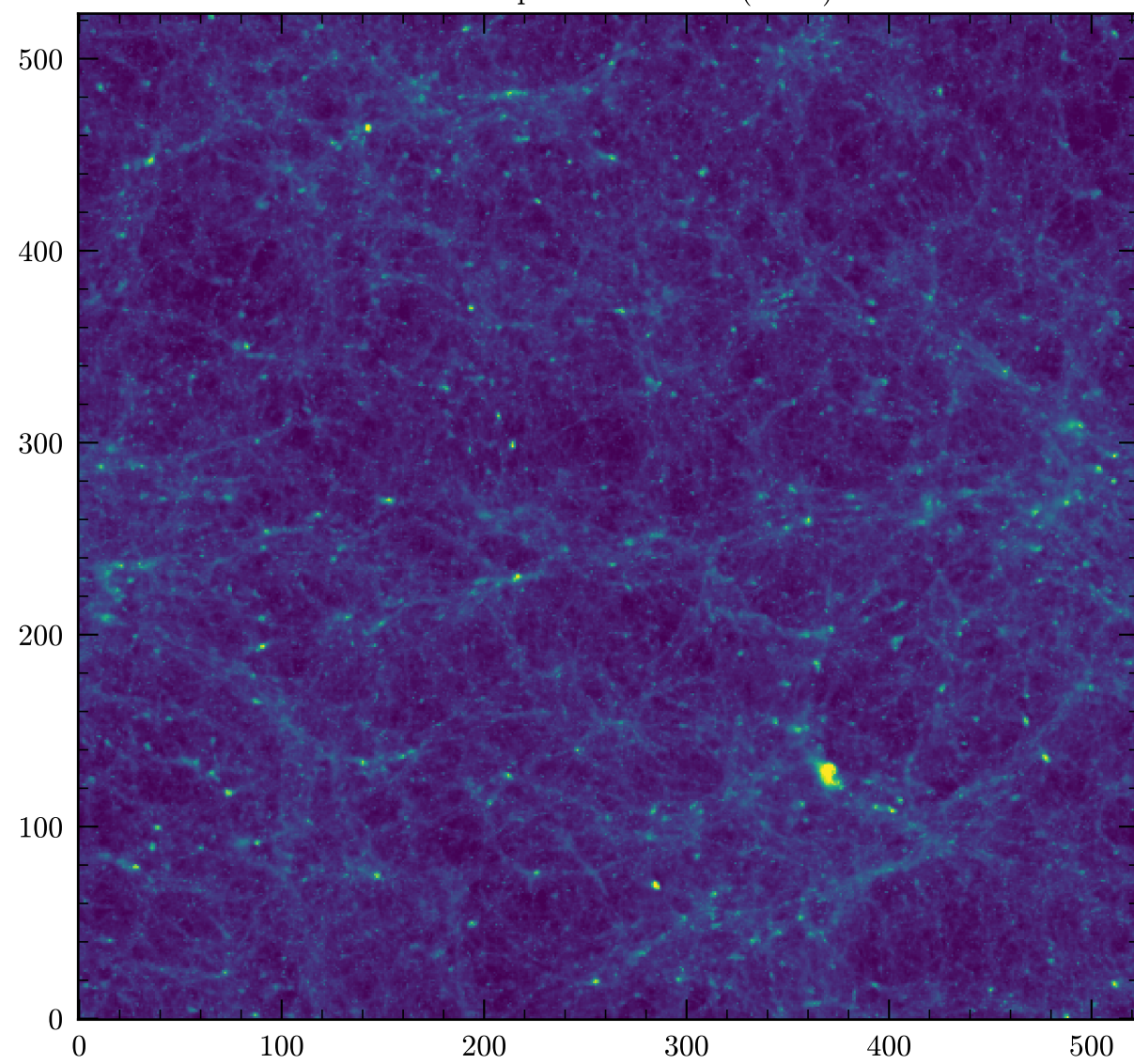
Recon Dispersion Measure (mean)
