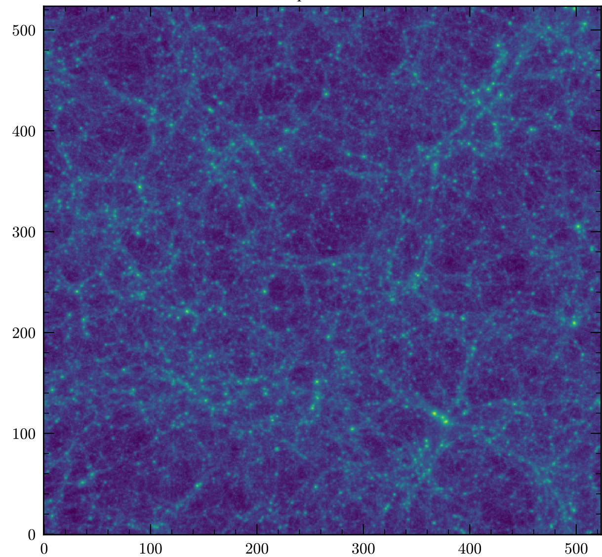
True Dispersion Measure
