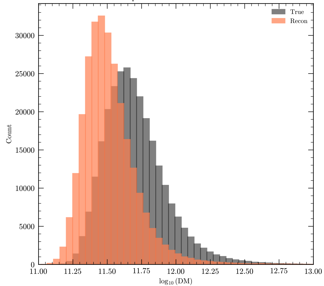
Dispersion Measure Distribution
