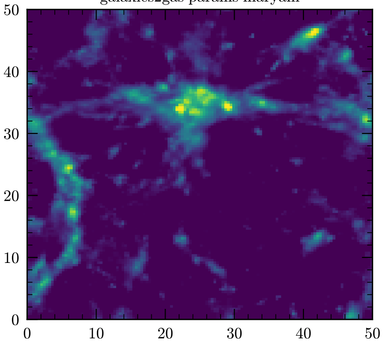
Dispersion Measure Distribution
