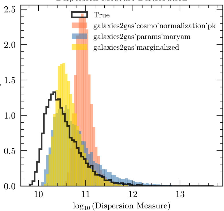
Dispersion Measure Distribution
