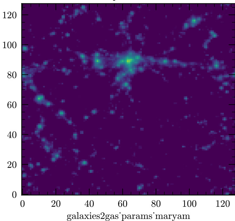
True Dispersion Measure
