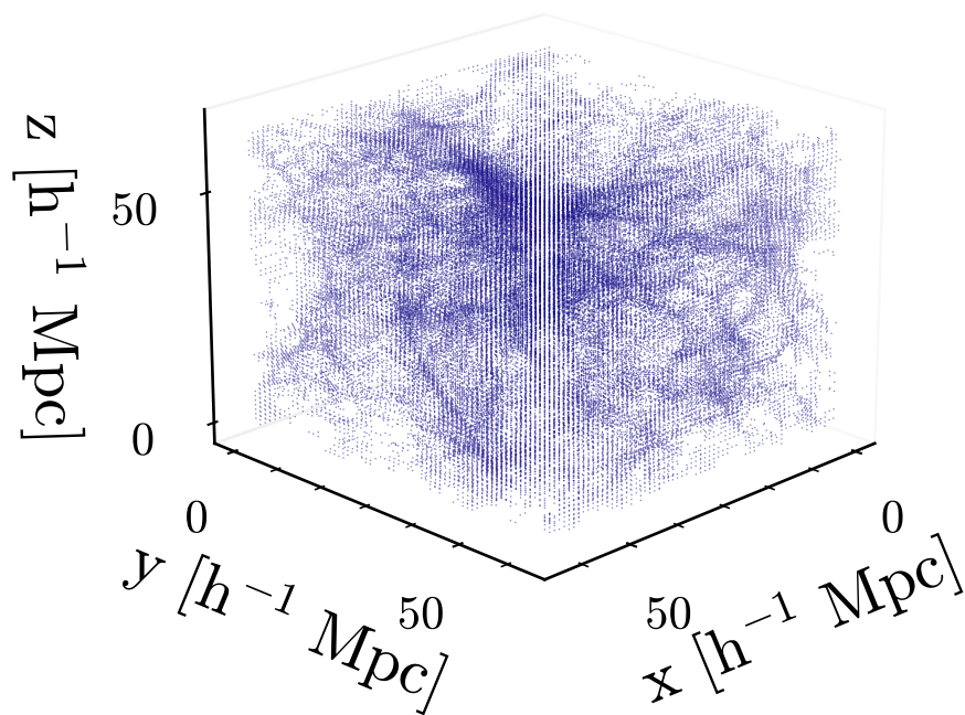
True Gas
