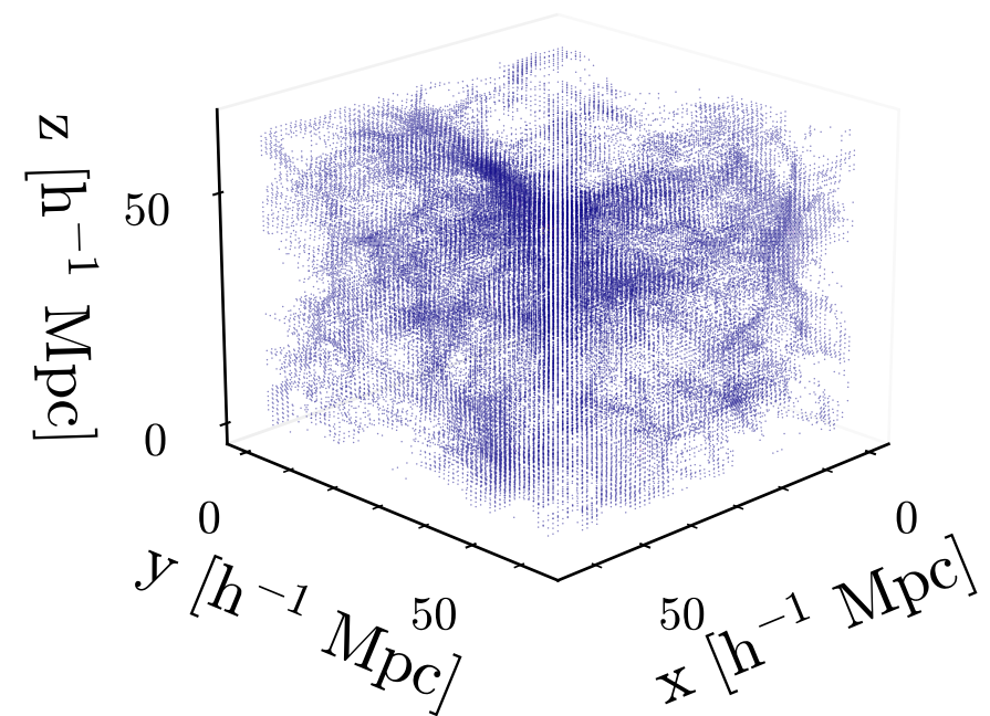
Reconstructed Gas
