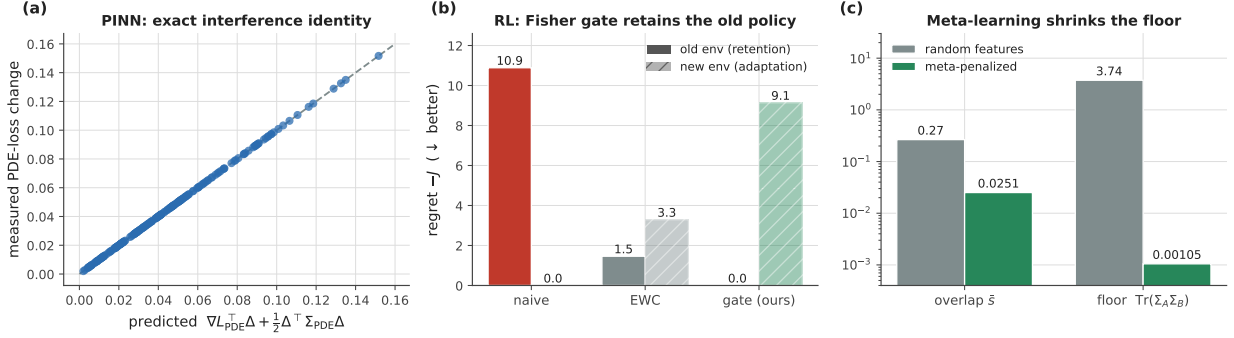
Figure S9: Three application domains for the interference functional ( evaluate_applications.py ). (a) Physics-informed regression: the interference identity with \Sigma_{PDE} predicts the measured PDE-loss change of data-only updates to machine precision (dashed: y = x ). (b) Policy gradients: routing the expected policy gradient orthogonal to the old environment’s Fisher subspace retains the old policy at zero regret while the new environment is learned in its free directions; naive descent forgets, and the Fisher-weighted anchor (the EWC analogue) is intermediate. (c) A feature map trained with the \text{Tr}(\Sigma_A \Sigma_B) penalty reduces inter-task overlap and the distortion-floor proxy by orders of magnitude (log scale), moving igfa into the lossless regime.
