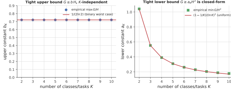
Figure S2: Tight multiclass entropy–variance constants for the floor sandwich, K = 2\text{--}10 . Left: \max_p G/H = 1/(2\ln 2) for every K (the binary posterior is the universal worst case). Right: \min_p G/H^2 = (1 - 1/K)/(\ln K)^2 , attained at the uniform posterior.
