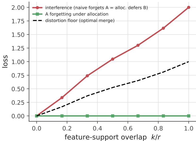
Interference is unavoidable iff supports overlap
