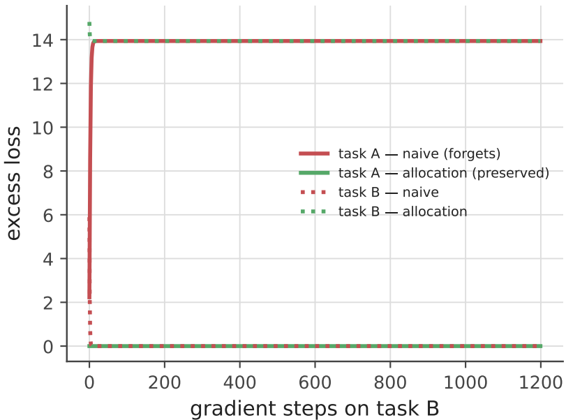
Allocation relocates cost: irreversible forgetting → deferred plasticity
