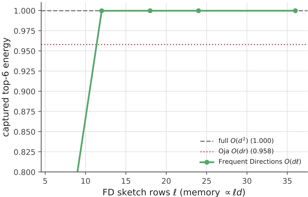
Cheap streaming subspace matches full at low memory
