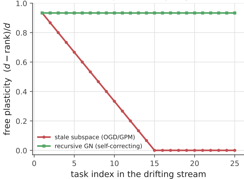
Re-estimation preserves capacity to learn
