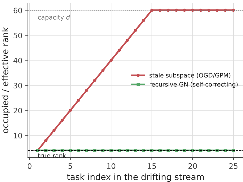
Stale projection exhausts capacity under drift
