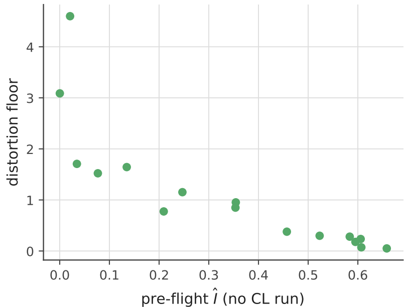
Probe forecasts the floor (monotone)
