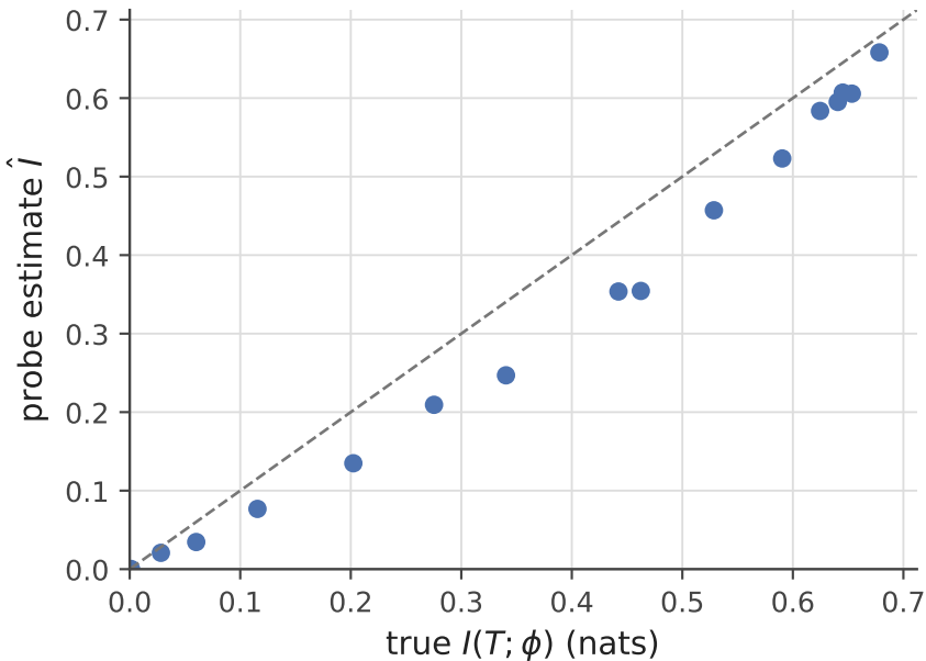
Cheap probe recovers MI ( r = 0.993 )
