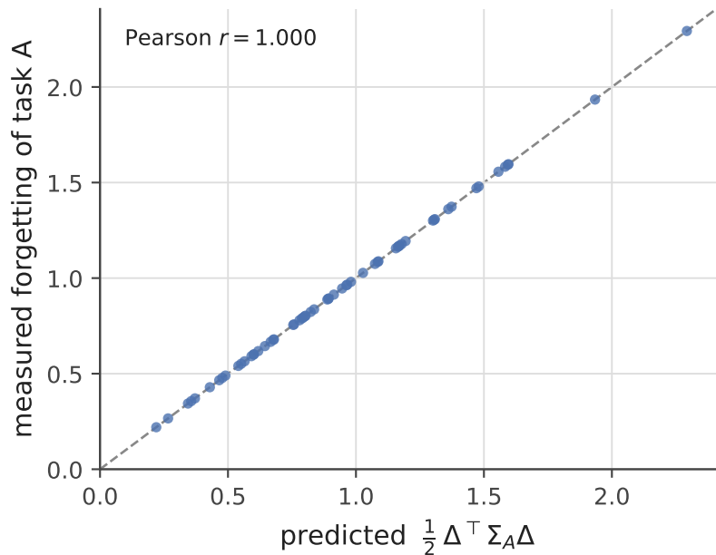
Nonlinear net: first-order prediction
