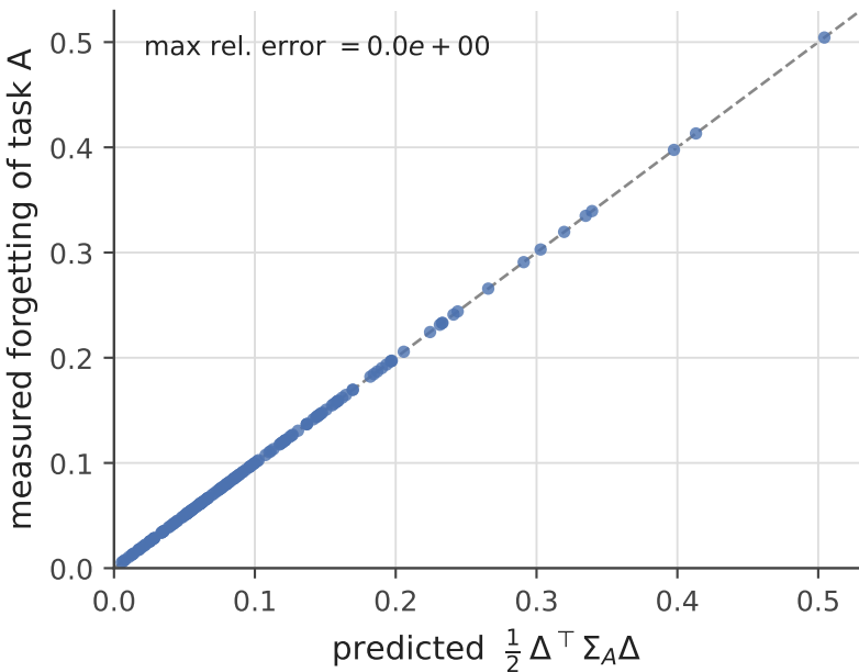
Linear head (frozen features): exact
