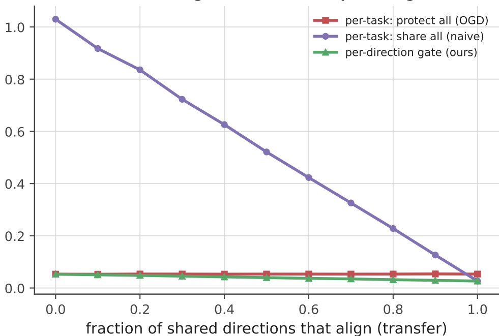
Per-direction gate dominates the per-task gate
