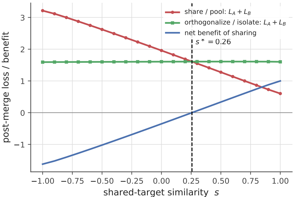
Sign-change: share above s^* , orthogonalize below
