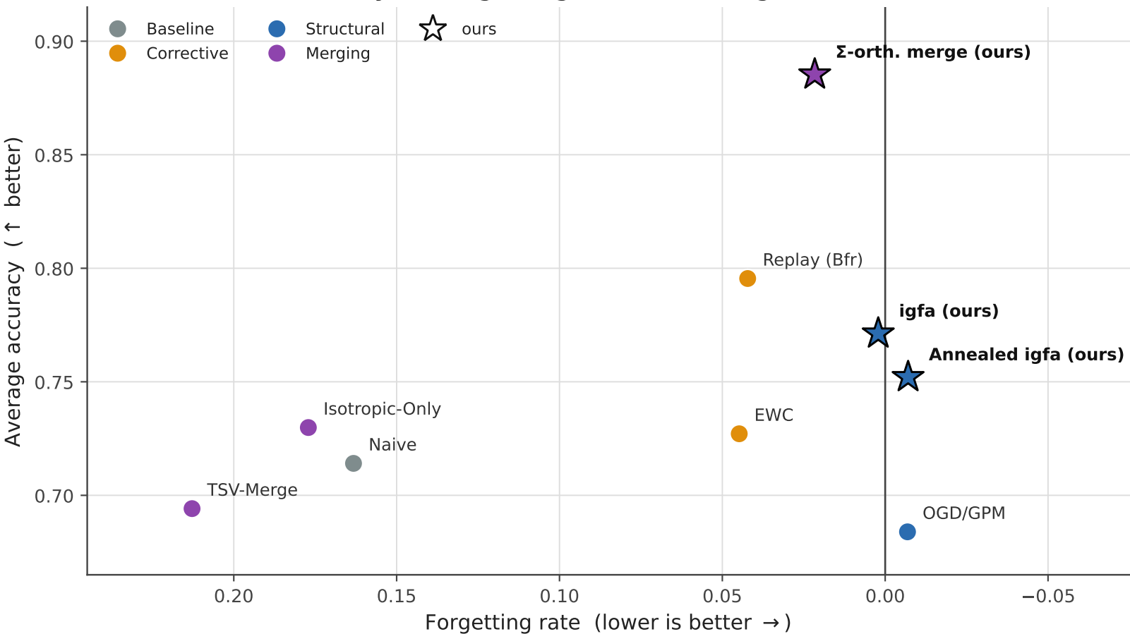
Accuracy vs. forgetting on Rotated-Digits (exact A1)
