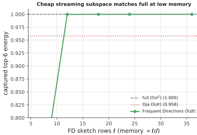
Figure S6: Cheap online Gauss–Newton subspace. Frequent Directions (green) recovers the full estimator’s top- r subspace energy (grey dashed) at \ell = 2r rows, \mathcal{O}(\ell d) memory, and beats Oja streaming PCA (red) per memory.
