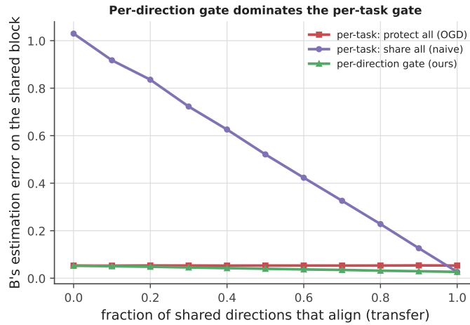
Figure S8: Per-direction vs per-task gating on a shared block, against the fraction of shared directions that align. The per-direction gate (green) follows the lower envelope—matching protect-all’s robustness and share-all’s transfer where each is right—while per-task share-all (purple) is catastrophic at low alignment.
