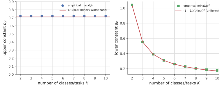
Figure S2: Tight multiclass entropy–variance constants for the floor sandwich, K = 2 – 10 . Left: \max_p G/H = 1/(2\ln 2) for every K (the binary posterior is the universal worst case). Right: \min_p G/H^2 = (1 - 1/K)/(\ln K)^2 , attained at the uniform posterior.
