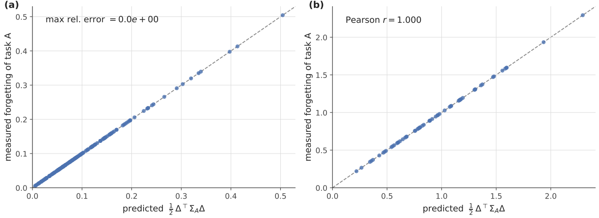
Figure 5: The interference functional is the forgetting. Measured backward-forgetting of task A against the predicted energy \frac{1}{2} \Delta^\top \Sigma_A \Delta . (a) A linear head on frozen features: the identity is exact to machine precision. (b) A nonlinear network, with the prediction formed from the last-layer feature covariance: first-order agreement, Pearson r > 0.9999 . The dashed line is y = x .
