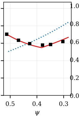
(c) NMC622
