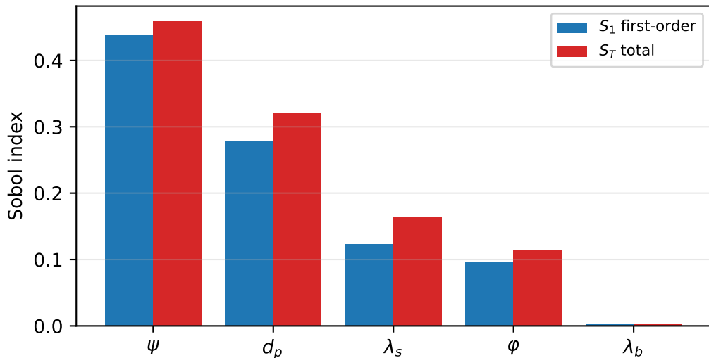
Sensitivity of dry-anode \lambda_{eff}
