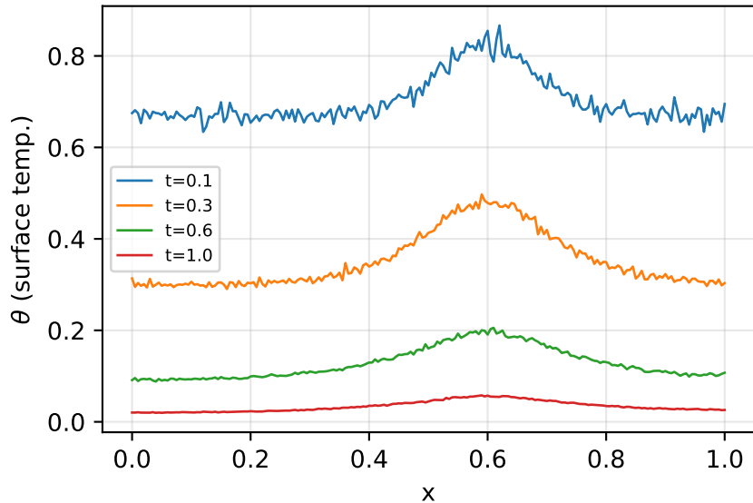
(a) synthetic IR frames (2% noise)
