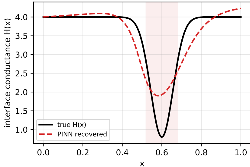
(b) recovered delamination field
