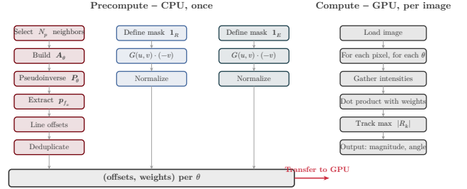
Fig. 14. Two-phase architecture overview. The precompute phase (left) runs on the CPU and differs per variant, but all three produce the same output format of (offset, weight) pairs per orientation. The compute phase (right) consumes these stencil arrays through a single variant-agnostic Triton kernel.
