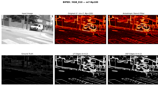
Fig. 19. Clean-data visual comparison on BIPED v1 (image 010). On this photometric-edge dataset, the ASF produces gradient maps visually competitive with deep learning outputs.
