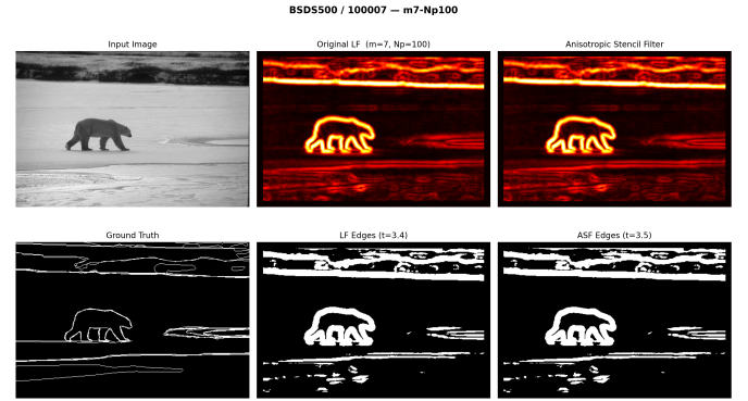
Fig. 16. Clean-data visual comparison on BSDS500 (image 100007). Top row: input image, naive LF gradient magnitude, ASF gradient magnitude (identical output, confirming mathematical equivalence). Bottom row: ground truth, LF edges, ASF edges.
