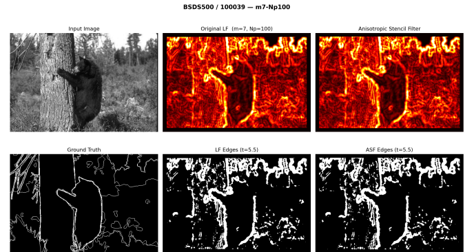
Fig. 17. Clean-data visual comparison on BSDS500 (image 100039). The ASF captures both strong object boundaries and fine internal texture edges.
