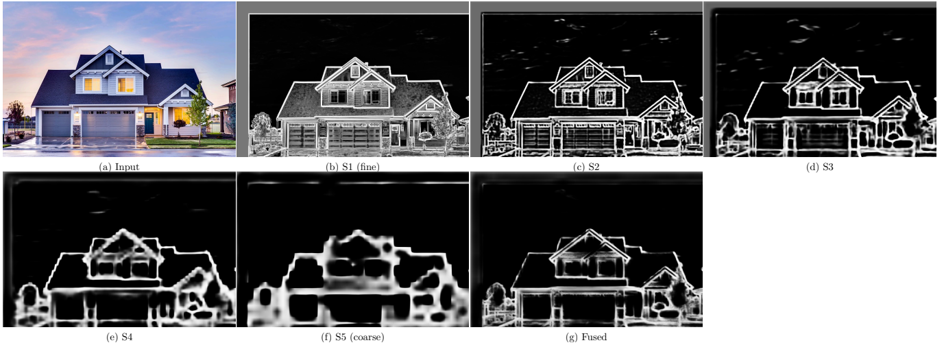
Fig. 25. HED side outputs and fused result. (a) Input image. (b)–(f) Side outputs S1 (finest) through S5 (coarsest), each produced by a different depth of the VGG-16 backbone and supervised independently during training. (g) The learned weighted fusion of all five side outputs. Fine-scale outputs respond to texture and thin lines; coarse-scale outputs respond to object boundaries and scene structure.
