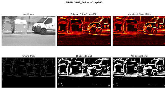
Fig. 18. Clean-data visual comparison on BIPED v1 (image 008, 1280 \times 720 ). The ASF captures fine structural details including vehicle outlines, wheel spokes, and sign text that small-kernel classical operators miss.
