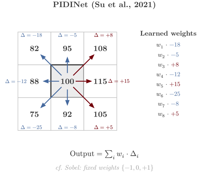
Fig. 9. PIDINet pixel difference convolutions (Su et al., 2021). Instead of multiplying pixel values by learned weights, PIDINet computes pixel differences \Delta_i between the center and each neighbor, then applies learned weights w_i to the differences. This is structurally similar to a classical gradient operator but with trainable coefficients.
