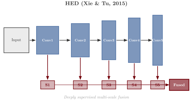
Fig. 8. Holistically-Nested Edge Detection (Xie and Tu, 2015). A VGG-style encoder produces multi-scale side outputs S_1 through S_5 that are fused into a final edge map. Each side output captures edges at a different spatial scale.
