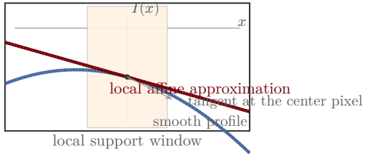
first-order local approximation
