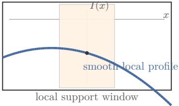
smooth intensity profile
