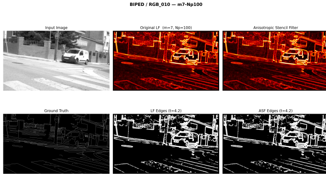
Fig. 19. Clean-data visual comparison on BIPED v1 (image 010). On this photometric-edge dataset, the ASF produces gradient maps visually competitive with deep learning outputs.
