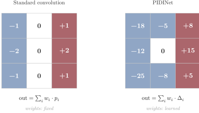
Fig. 9. PIDINet pixel difference convolutions (Su et al., 2021). Instead of multiplying pixel values by learned weights, PIDINet computes pixel differences \Delta_i between the center and each neighbor, then applies learned weights w_i to the differences. This is structurally similar to a classical gradient operator but with trainable coefficients.
