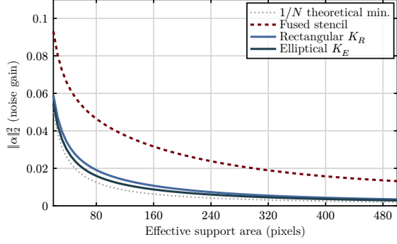
Fig. 13. Noise gain \|\alpha\|_2^2 as a function of effective support area for the three kernel variants. The theoretical minimum for a uniform kernel ( 1/N ) is shown as a dotted line. The geometric kernels track closer to the theoretical minimum across all support sizes. The fused stencil curve sits above due to its uneven weight distribution.
