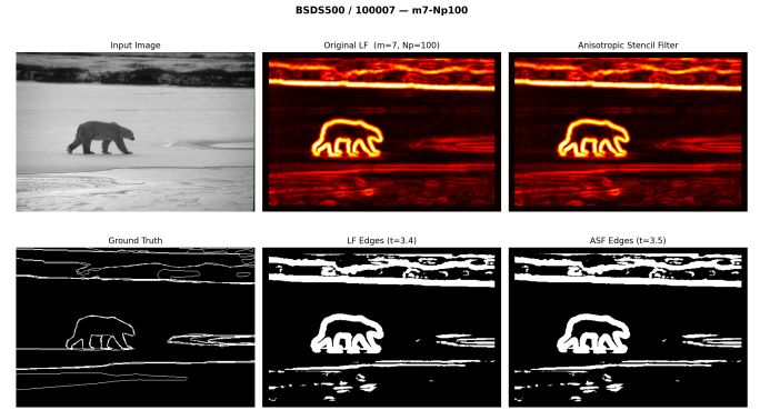
Fig. 16. Clean-data visual comparison on BSDS500 (image 100007). Top row: input image, naive LF gradient magnitude, ASF gradient magnitude (identical output, confirming mathematical equivalence). Bottom row: ground truth, LF edges, ASF edges.
