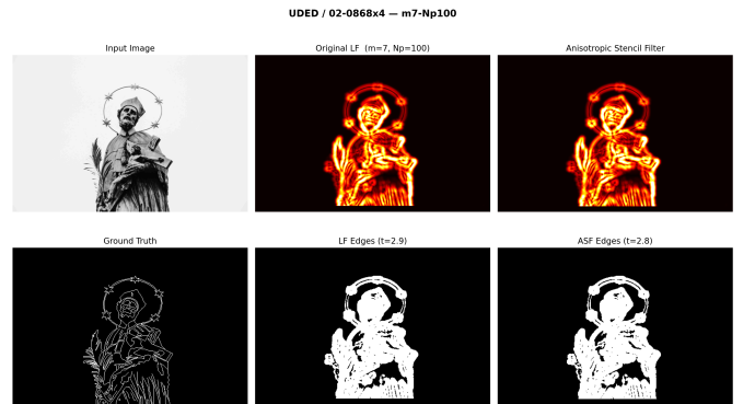
Fig. 34. Clean-data visual comparison on UDED (image 02). On this cross-domain benchmark, the ASF approaches DexiNed’s supervised performance without any training data.
