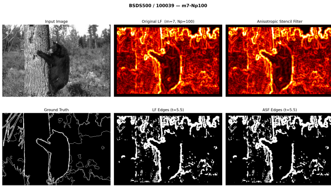
Fig. 30. Clean-data visual comparison on BSDS500 (image 100039). The ASF captures both strong object boundaries and fine internal texture edges.
