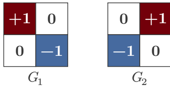
Fig. 10. Roberts Cross operator (1963). Two 2 \times 2 kernels compute diagonal intensity differences. Positive weights in garnet, negative in blue.
