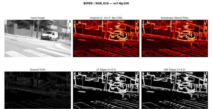
Fig. 24. Clean-data visual comparison on BIPED v1 (image 010). On this photometric-edge dataset, the ASF produces gradient maps visually competitive with deep learning outputs.
