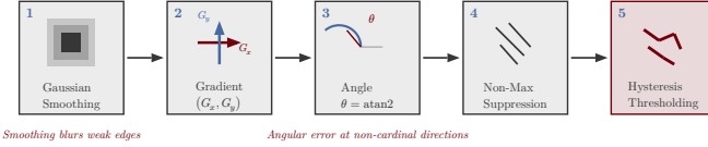
Fig. 8. The Canny edge detection pipeline (1986). Five stages: Gaussian smoothing, gradient computation, angle estimation via arctan, non-maximum suppression, and hysteresis thresholding. The pre-smoothing step trades edge localization for noise robustness; stronger smoothing blurs weak edges.
