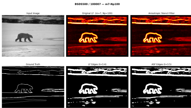
Fig. 21. Clean-data visual comparison on BSDS500 (image 100007). Top row: input image, naive LF gradient magnitude, ASF gradient magnitude (identical output, confirming mathematical equivalence). Bottom row: ground truth, LF edges, ASF edges.
