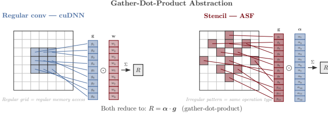
Fig. 11. The gather-dot-product abstraction. Both regular convolution (left, as in cuDNN) and irregular stencil operations (right, as in the ASF) reduce to the same primitive: gather pixel intensities at precomputed offsets, multiply by precomputed weights, and sum. This uniformity enables a single GPU kernel to serve all three proposed filter variants.
