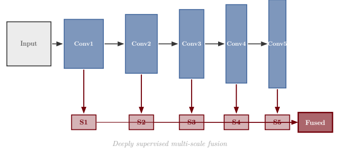
Fig. 9. Holistically-Nested Edge Detection (Xie and Tu, 2015). A VGG-style encoder produces multi-scale side outputs S_1 through S_5 that are fused into a final edge map. Each side output captures edges at a different spatial scale.
