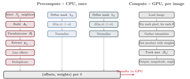
Fig. 19. Two-phase architecture overview. The precompute phase (left) runs on the CPU and differs per variant, but all three produce the same output format of (offset, weight) pairs per orientation. The compute phase (right) consumes these stencil arrays through a single variant-agnostic Triton kernel.
