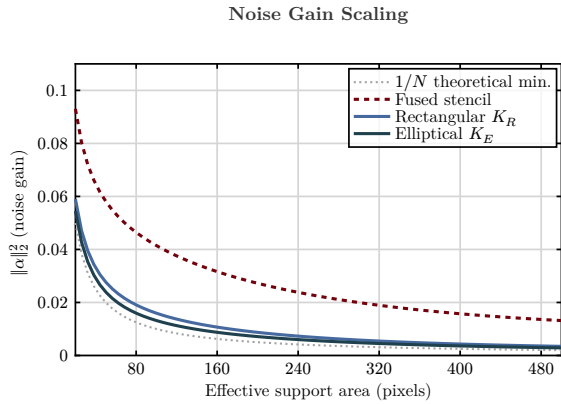
Fig. 18. Noise gain \|\alpha\|_2^2 as a function of effective support area for the three kernel variants. The theoretical minimum for a uniform kernel ( 1/N ) is shown as a dotted line. The geometric kernels track closer to the theoretical minimum across all support sizes. The fused stencil curve sits above due to its uneven weight distribution.
