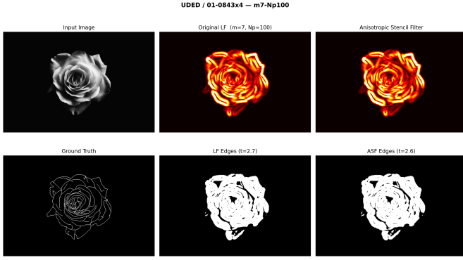
Fig. 25. Clean-data visual comparison on UDED (image 01). The ASF generalizes across diverse imaging domains without domain-specific training, detecting boundaries and internal structure.
