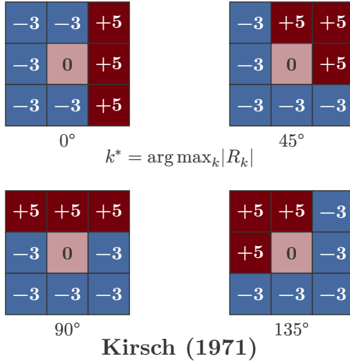
Fig. 13. Kirsch compass operator (1971). Four of the eight 3 \times 3 compass masks are shown at 0^\circ , 45^\circ , 90^\circ , and 135^\circ . The edge response is the maximum over all eight orientations, an early instance of the orientation sweep that the WVF later employs with polynomial fitting.
