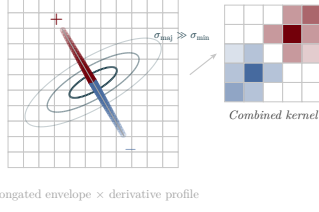
Fig. 8. Anisotropic Gaussian derivatives (Geusebroek et al., 2003). An elongated Gaussian envelope aligned along the candidate edge direction is modulated by the normal derivative profile ( -v ), producing the dipole pattern that is essentially identical to the geometric kernels proposed in this work.
