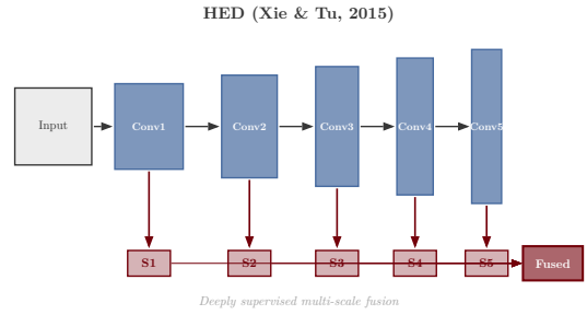
Fig. 17. Holistically-Nested Edge Detection (Xie and Tu, 2015). A VGG-style encoder produces multi-scale side outputs S_1 through S_5 that are fused into a final edge map. Each side output captures edges at a different spatial scale.
