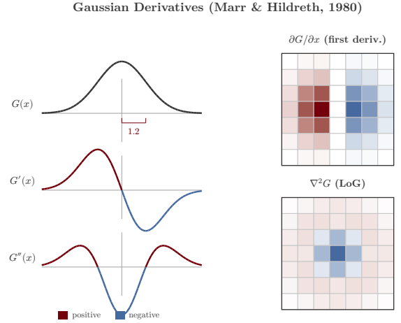
Fig. 15. Gaussian derivatives. Left: the Gaussian function G(x) , its first derivative G'(x) (odd-symmetric dipole), and its second derivative G''(x) (Mexican hat). Right: the corresponding 2D kernels. The first-derivative-of-Gaussian kernel is the mathematical ancestor of the geometric kernels proposed in this work.
