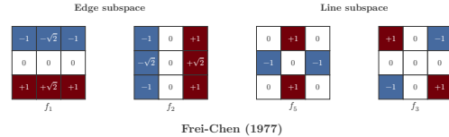
Fig. 14. Frei-Chen operator (1977). The 3 \times 3 neighborhood is decomposed into orthogonal subspaces. Representative edge-subspace and line-subspace basis masks are shown. Edges are detected by projecting the image patch onto the edge subspace.
