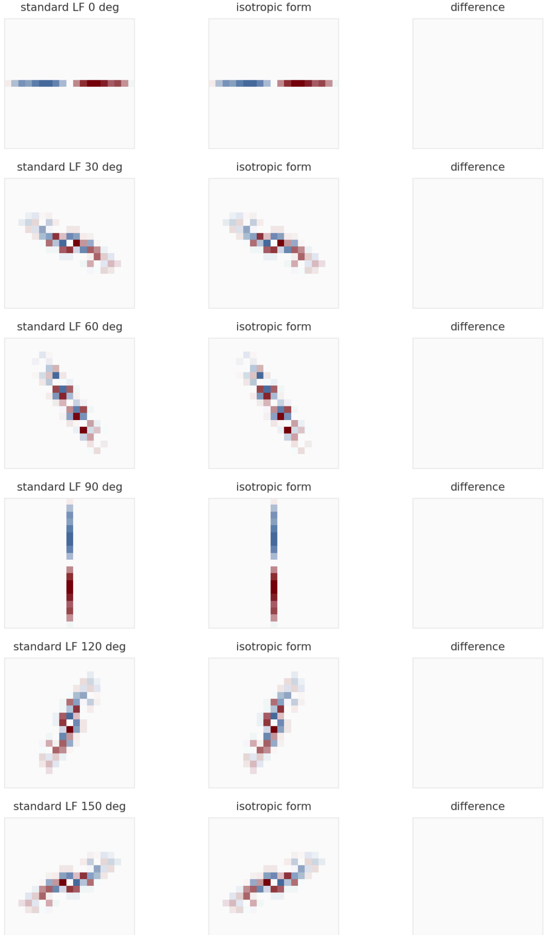
Figure 2: Standard LF kernels compared with kernels rebuilt from one isotropic \frac{G_x}{G_y} pair plus oriented line smoothing. The maximum absolute kernel difference over the full 36-angle bank is 1.03 \times 10^{-15} .
