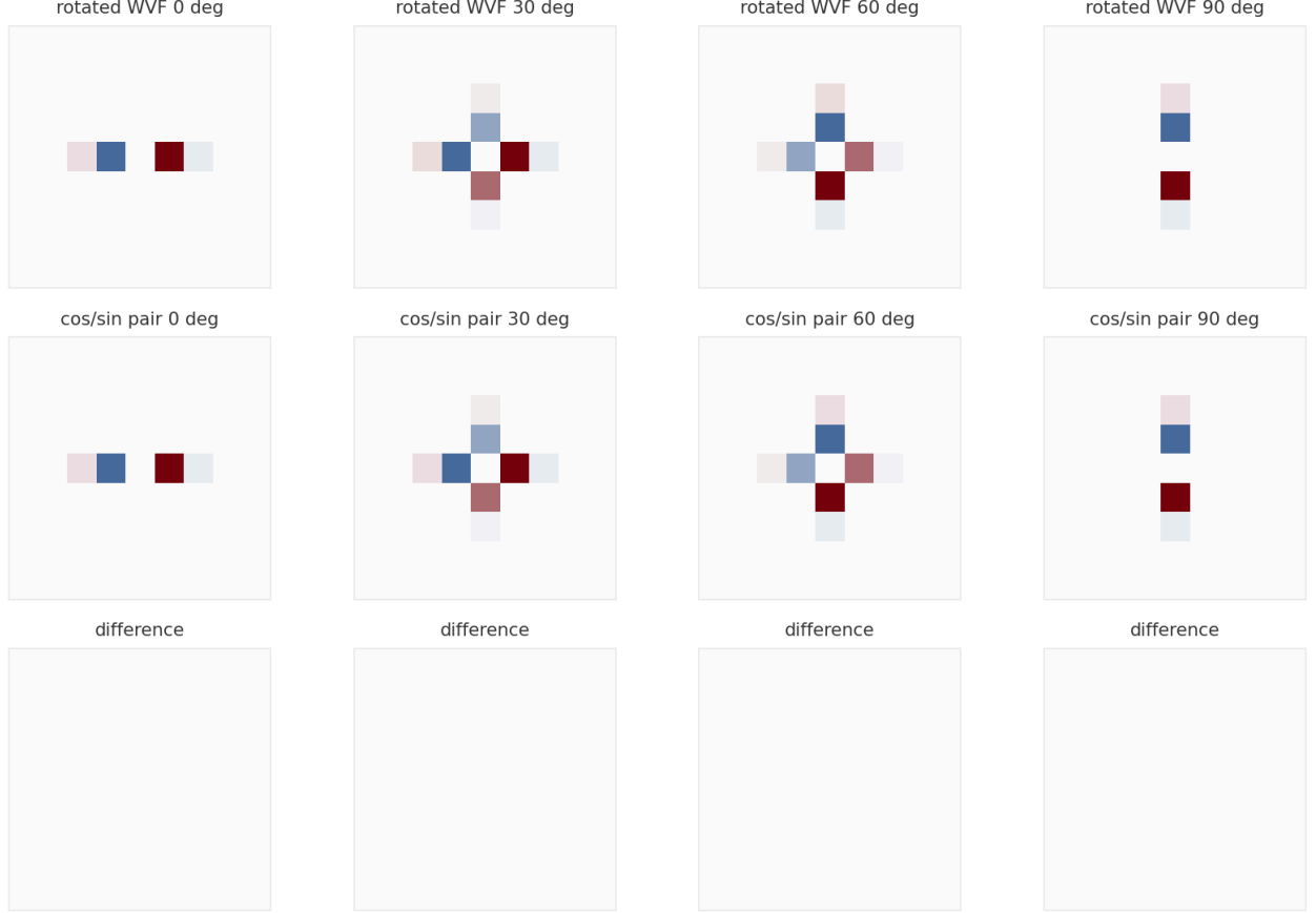
Figure 1: A numerical check of Equation 2.3 for the local Taylor/WVF derivative rows. The first row shows derivative kernels obtained by rotating the WVF coordinates. The second row shows the same kernels reconstructed from one isotropic G_x and G_y pair. The third row shows the difference.
