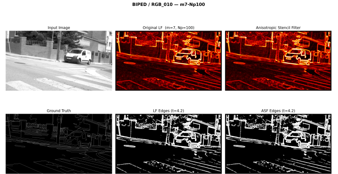
Fig. 32. Clean-data visual comparison on BIPED v1 (image 010). On this photometric-edge dataset, the ASF produces gradient maps visually competitive with deep learning outputs.
