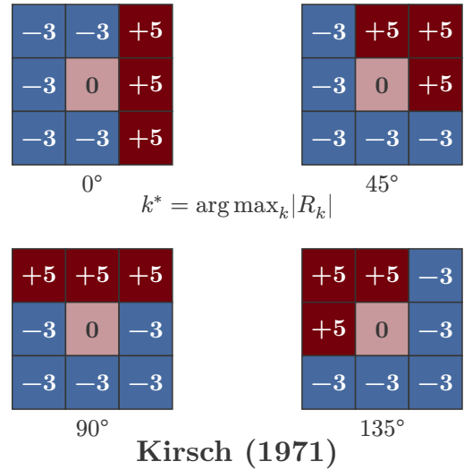
Fig. 13. Kirsch compass operator (1971). Four of the eight 3 \times 3 compass masks are shown at 0^\circ , 45^\circ , 90^\circ , and 135^\circ . The edge response is the maximum over all eight orientations, an early instance of the orientation sweep that the WVF later employs with polynomial fitting.
