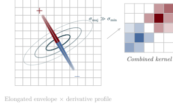
Fig. 8. Anisotropic Gaussian derivatives (Geusebroek et al., 2003). An elongated Gaussian envelope aligned along the candidate edge direction is modulated by the normal derivative profile ( -v ), producing the dipole pattern that is essentially identical to the geometric kernels proposed in this work.
