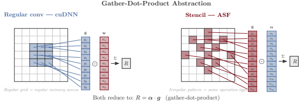
Fig. 19. The gather-dot-product abstraction. Both regular convolution (left, as in cuDNN) and irregular stencil operations (right, as in the ASF) reduce to the same primitive: gather pixel intensities at precomputed offsets, multiply by precomputed weights, and sum. This uniformity enables a single GPU kernel to serve all three proposed filter variants.
