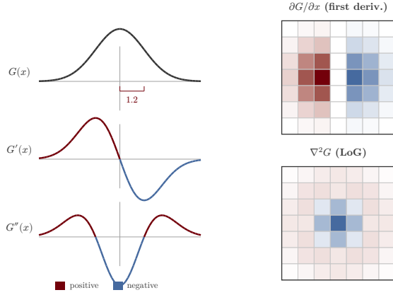
Fig. 15. Gaussian derivatives. Left: the Gaussian function G(x) , its first derivative G'(x) (odd-symmetric dipole), and its second derivative G''(x) (Mexican hat). Right: the corresponding 2D kernels. The first-derivative-of-Gaussian kernel is the mathematical ancestor of the geometric kernels proposed in this work.
