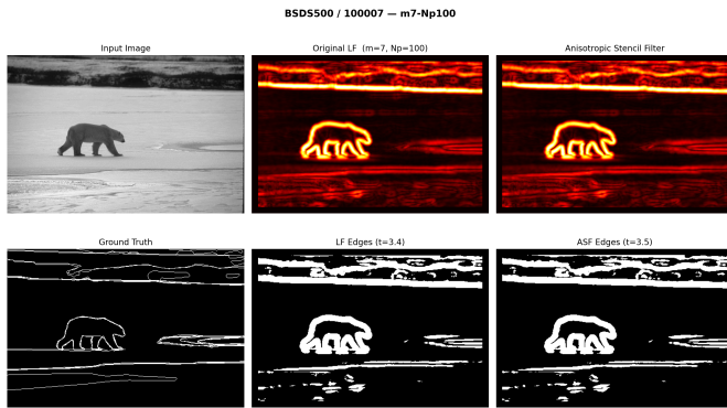
Fig. 29. Clean-data visual comparison on BSDS500 (image 100007). Top row: input image, naive LF gradient magnitude, ASF gradient magnitude (identical output, confirming mathematical equivalence). Bottom row: ground truth, LF edges, ASF edges.
