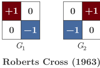
Fig. 10. Roberts Cross operator (1963). Two 2 \times 2 kernels compute diagonal intensity differences. Positive weights in garnet, negative in blue.
