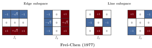
Fig. 14. Frei–Chen operator (1977). The 3 \times 3 neighborhood is decomposed into orthogonal subspaces. Representative edge-subspace and line-subspace basis masks are shown. Edges are detected by projecting the image patch onto the edge subspace.
