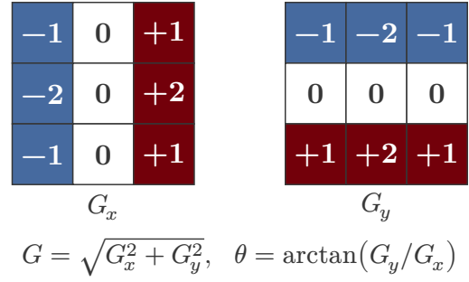
Sobel (1968)
