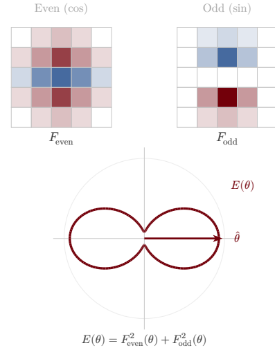
Fig. 7. Oriented energy (Morrone and Owens, 1987). Even-symmetric and odd-symmetric filter pairs are combined to form the local energy E(\theta) = F_{\text{even}}^2 + F_{\text{odd}}^2 , whose peak indicates the dominant edge orientation.
