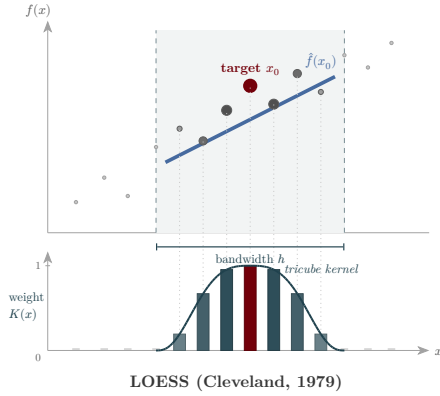
Fig. 3. LOESS (Cleveland, 1979). Data points are weighted by a distance-based kernel centered on the target point; nearer samples (larger dots) contribute more strongly to the local polynomial fit.
