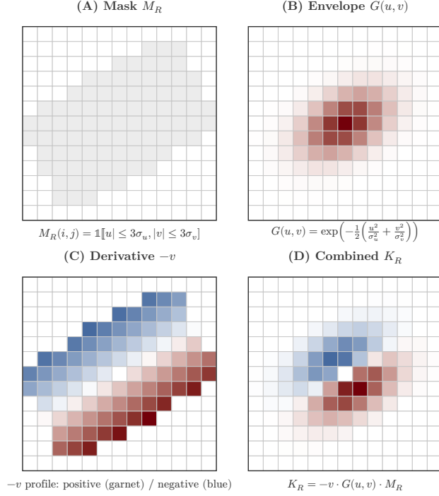
Fig. 23. Construction of the rectangular Gaussian kernel at \theta = 30^\circ . (A) The rectangular mask region on the pixel grid, with interior pixels highlighted. (B) The anisotropic Gaussian envelope within the mask, darker at the center and lighter toward the boundary. (C) The derivative profile -v shown as a cross-section, with positive values above the center line and negative values below. (D) The final combined kernel K_R , with each cell colored by its weight magnitude and sign. The dipole pattern is clean and regular, with no near-zero interior pixels.
