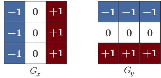
Prewitt (1970)
