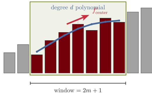
Fig. 1. One-dimensional Savitzky–Golay filtering. A polynomial of degree d is fitted to a sliding window of 2m + 1 samples (highlighted), and the derivative at the center point is extracted from the fitted coefficients.
