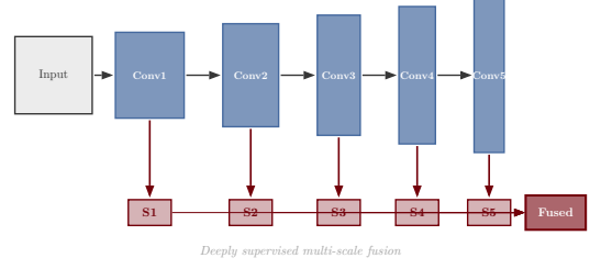
Fig. 17. Holistically-Nested Edge Detection (Xie and Tu, 2015). A VGG-style encoder produces multi-scale side outputs S_1 through S_5 that are fused into a final edge map. Each side output captures edges at a different spatial scale.
