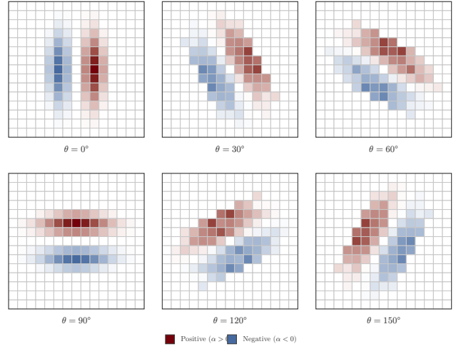
Fig. 10. Fused weight maps \alpha_{k,\ell} computed from the pseudoinverse for six orientations ( m = 4 , N_p = 29 , d = 2 ). Garnet indicates positive weights and blue indicates negative weights, with intensity proportional to magnitude. The dipole pattern rotates with \theta_k and the stencil elongates along the candidate edge tangent. At grid-aligned orientations ( \theta = 0^\circ, 90^\circ ), adjacent line positions land on exact integer offsets, producing maximal neighborhood overlap and the most severe weight cancellation (visible as washed-out cells between the positive and negative lobes).
