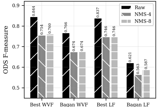
Fig. 6. Effect of non-maximum suppression (NMS) on ODS for various WVF and LF configurations on BIPED. Both 4-directional and 8-directional NMS consistently reduce ODS compared to the raw gradient magnitude output.
