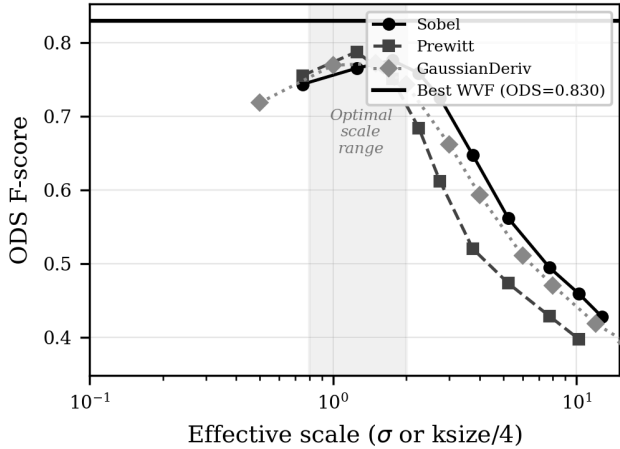
Fig. 2. ODS vs. scale parameter for each classical operator family on BIPED v1. Each family shows a clear optimal scale, with performance degrading sharply at both extremes.
