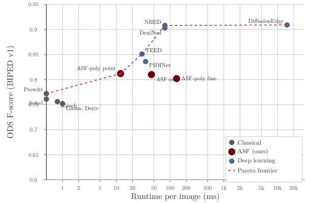
Fig. 24. Accuracy vs. runtime Pareto plot on BIPED v1. Classical methods (gray) cluster at low runtime but low accuracy. Deep learning models (blue) achieve high accuracy at higher computational cost. The ASF variants (garnet) occupy the previously empty region, offering accuracy competitive with lightweight neural networks at classical-method runtimes.
