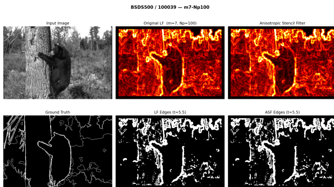
Fig. 17. Clean-data visual comparison on BSDS500 (image 100039). The ASF captures both strong object boundaries and fine internal texture edges.
