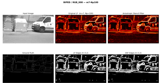
Fig. 18. Clean-data visual comparison on BIPED v1 (image 008, 1280 \times 720 ). The ASF captures fine structural details including vehicle outlines, wheel spokes, and sign text that small-kernel classical operators miss.
