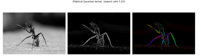
Fig. 23. Elliptical Gaussian kernel edge detection on the same image. The gradient magnitude map is visually nearly identical to the rectangular variant. The orientation field is slightly smoother, consistent with the elliptical kernel’s continuous angular weighting.
