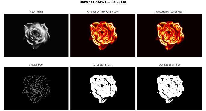
Fig. 33. Clean-data visual comparison on UDED (image 01). The ASF generalizes across diverse imaging domains without domain-specific training, detecting boundaries and internal structure.
