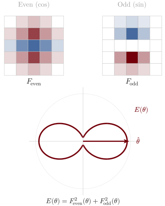
Fig. 7. Oriented energy (Morrone and Owens, 1987). Even-symmetric and odd-symmetric filter pairs are combined to form the local energy E(\theta) = F_{\text{even}}^2 + F_{\text{odd}}^2 , whose peak indicates the dominant edge orientation.
