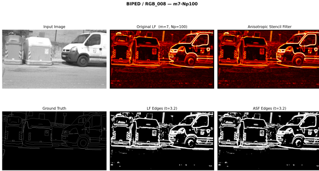
Fig. 31. Clean-data visual comparison on BIPED v1 (image 008, 1280 \times 720 ). The ASF captures fine structural details including vehicle outlines, wheel spokes, and sign text that small-kernel classical operators miss.
