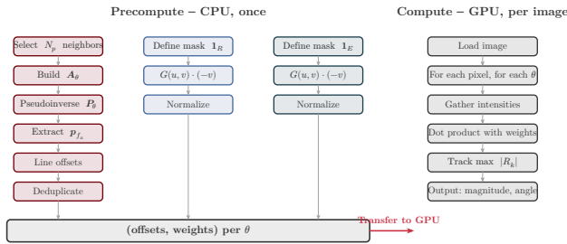
Fig. 27. Two-phase architecture overview. The precompute phase (left) runs on the CPU and differs per variant, but all three produce the same output format of (offset, weight) pairs per orientation. The compute phase (right) consumes these stencil arrays through a single variant-agnostic Triton kernel.
