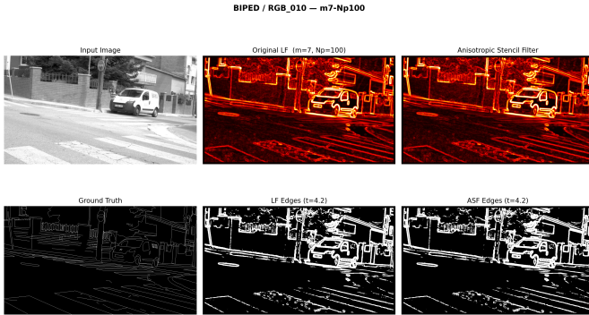
Fig. 32. Clean-data visual comparison on BIPED v1 (image 010). On this photometric-edge dataset, the ASF produces gradient maps visually competitive with deep learning outputs.
