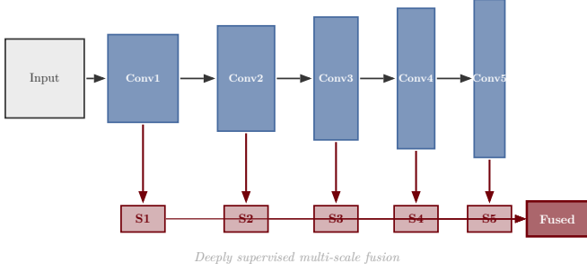
Fig. 17. Holistically-Nested Edge Detection (Xie and Tu, 2015). A VGG-style encoder produces multi-scale side outputs S_1 through S_5 that are fused into a final edge map. Each side output captures edges at a different spatial scale.
