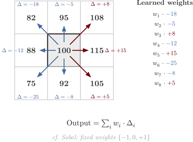
Fig. 18. PIDINet pixel difference convolutions (Su et al., 2021). Instead of multiplying pixel values by learned weights, PIDINet computes pixel differences \Delta_i between the center and each neighbor, then applies learned weights w_i to the differences. This is structurally similar to a classical gradient operator but with trainable coefficients.
