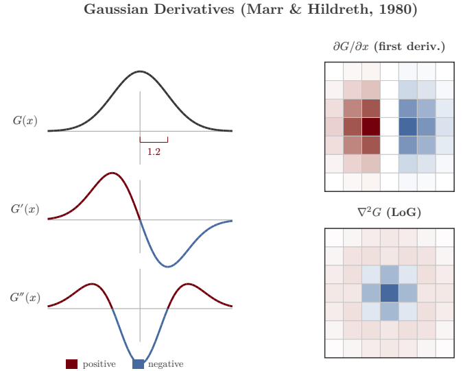
Fig. 15. Gaussian derivatives. Left: the Gaussian function G(x) , its first derivative G'(x) (odd-symmetric dipole), and its second derivative G''(x) (Mexican hat). Right: the corresponding 2D kernels. The first-derivative-of-Gaussian kernel is the mathematical ancestor of the geometric kernels proposed in this work.
