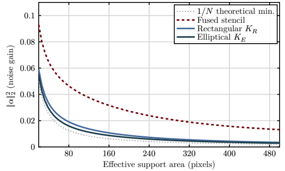
Fig. 26. Noise gain \|\alpha\|_2^2 as a function of effective support area for the three kernel variants. The theoretical minimum for a uniform kernel ( 1/N ) is shown as a dotted line. The geometric kernels track closer to the theoretical minimum across all support sizes. The fused stencil curve sits above due to its uneven weight distribution.
