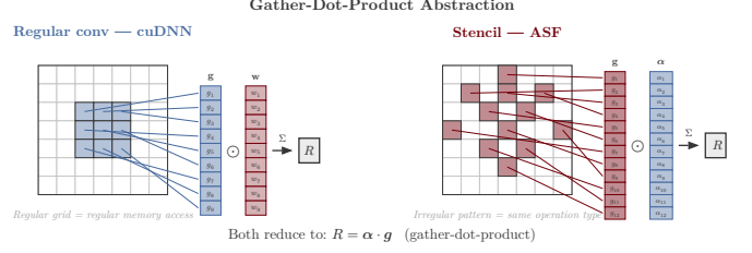
Fig. 19. The gather-dot-product abstraction. Both regular convolution (left, as in cuDNN) and irregular stencil operations (right, as in the ASF) reduce to the same primitive: gather pixel intensities at precomputed offsets, multiply by precomputed weights, and sum. This uniformity enables a single GPU kernel to serve all three proposed filter variants.
