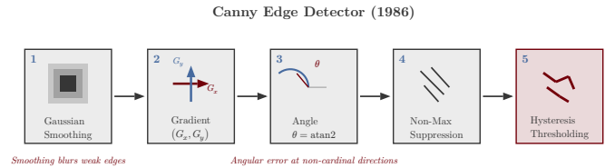
Fig. 16. The Canny edge detection pipeline (1986). Five stages: Gaussian smoothing, gradient computation, angle estimation via arctan, non-maximum suppression, and hysteresis thresholding. The pre-smoothing step trades edge localization for noise robustness; stronger smoothing blurs weak edges.
