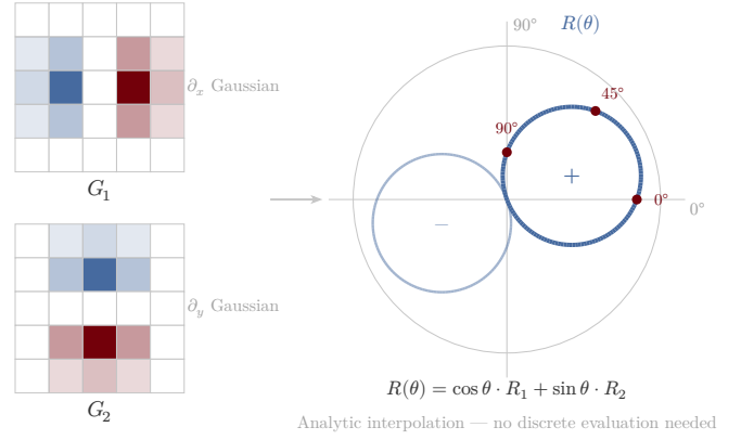
Fig. 6. Steerable filters (Freeman and Adelson, 1991). Two basis kernels G_1 and G_2 (first derivatives of a Gaussian in the x and y directions) are combined as R(\theta) = \cos(\theta)R_1 + \sin(\theta)R_2 to analytically interpolate the response at any orientation, without discrete evaluation.
