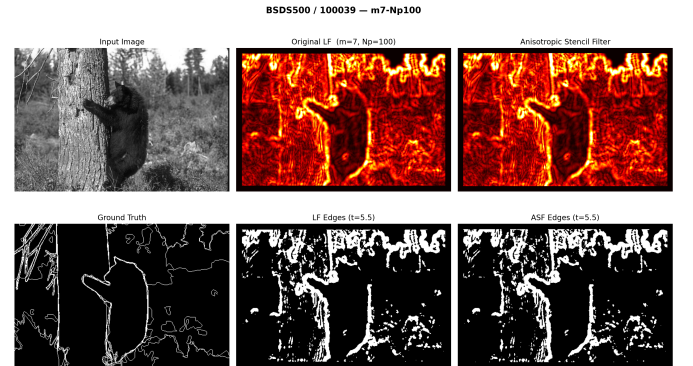
Fig. 30. Clean-data visual comparison on BSDS500 (image 100039). The ASF captures both strong object boundaries and fine internal texture edges.
