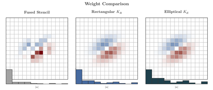
Fig. 25. Side-by-side weight comparison at \theta = 30^\circ for the three kernel variants. Left: the fused stencil weight map, showing an irregular shape with many near-zero cells. Center: the rectangular kernel, exhibiting a clean box boundary and smooth dipole weights with no near-zero interior pixels. Right: the elliptical kernel, with a smooth elliptical boundary and slightly fewer pixels. Below each weight map is a histogram of absolute weight magnitudes |\alpha| . The fused stencil histogram exhibits a pronounced spike near zero; neither geometric kernel histogram does.
