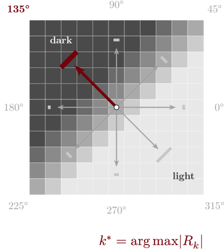
Fig. 9. Discrete orientation sweep as used by the WVF and the proposed ASF. Eight candidate orientations are evaluated; the response magnitude at each angle is indicated by the bar height. The orientation with maximum response (highlighted) is selected as the edge direction. This is a brute-force approximation of the analytic steering shown in Fig. 6.
