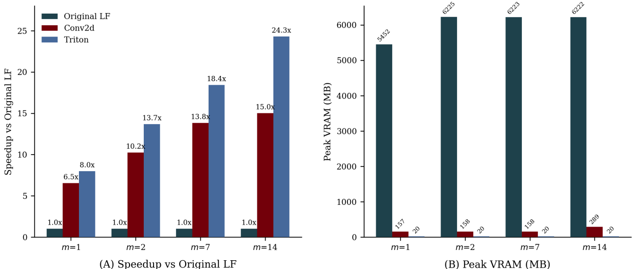
Figure 4: GPU performance on BIPED v1 (1280×720). (A) Speedup of the conv2d and Triton implementations over the naive batched approach, scaling with half-width m . (B) Peak VRAM consumption; the Triton kernel uses only 20 MB regardless of m , a 311× reduction.
