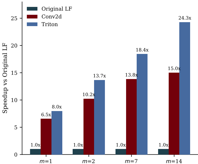
(A) Speedup vs Original LF
