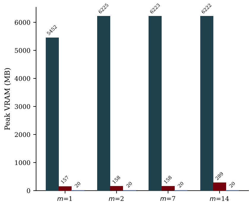
(B) Peak VRAM (MB)
