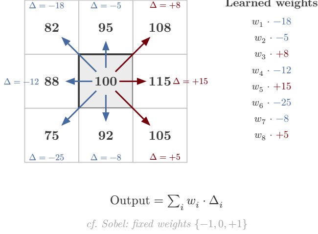
Fig. 9. PIDINet pixel difference convolutions (Su et al., 2021). Instead of multiplying pixel values by learned weights, PIDINet computes pixel differences \Delta_i between the center and each neighbor, then applies learned weights w_i to the differences. This is structurally similar to a classical gradient operator but with trainable coefficients.
