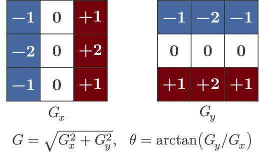
Fig. 11. Sobel operator (1968). Two 3 \times 3 kernels G_x and G_y estimate horizontal and vertical gradients with center-weighted smoothing. The gradient magnitude and direction are obtained by combining both responses.
