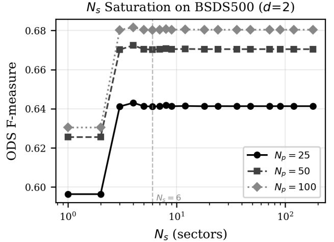
Fig. 3. ODS versus orientation count N_s at several fixed N_p values ( d = 2 ). Performance saturates by N_s = 4\text{--}6 , with negligible improvement from the published N_s = 18 or beyond.
