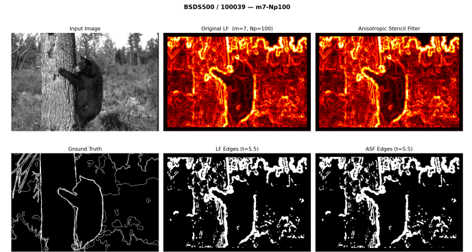
Fig. 20. Clean-data visual comparison on BSDS500 (image 100039). The ASF captures both strong object boundaries and fine internal texture edges.
