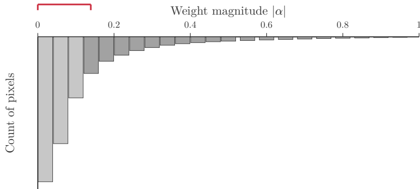
Distribution of fused stencil weight magnitudes ( m = 7 , N_p = 15 )
