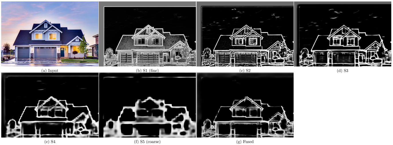
Fig. 27. HED side outputs and fused result. (a) Input image. (b)–(f) Side outputs S1 (finest) through S5 (coarsest), each produced by a different depth of the VGG-16 backbone and supervised independently during training. (g) The learned weighted fusion of all five side outputs. Fine-scale outputs respond to texture and thin lines; coarse-scale outputs respond to object boundaries and scene structure.
