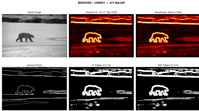
Fig. 18. Clean-data visual comparison on BSDS500 (image 100007). Top row: input image, naive LF gradient magnitude, ASF gradient magnitude (identical output, confirming mathematical equivalence). Bottom row: ground truth, LF edges, ASF edges.
