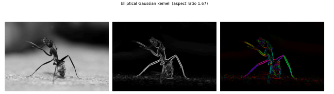
Fig. 25. Elliptical Gaussian kernel edge detection on the same image. The gradient magnitude map is visually nearly identical to the rectangular variant. The orientation field is slightly smoother, consistent with the elliptical kernel’s continuous angular weighting.
